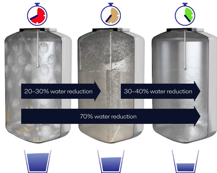
Savings using three different tank cleaning systems: spray ball, rotary spray head and rotary jet head.
